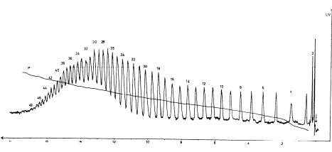
Figure 8. Separation of polystyrene 2200 with pressure programming by Klesper and Hartmann in 1977. Mobile phase: n-pentane with 10% methanol.
