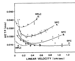
Figure 9. HETP vs. linear velocity: curve A, data from SFC on 10 \mu\text{m} packing; curve B, SFC on 5 \mu\text{m} ; curve C, SFC on 3 \mu\text{m} ; curve D, HPLC on 10 \mu\text{m} ; curve E, HPLC on 3 \mu\text{m} .
