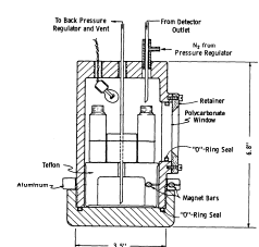
Figure 6. Pressurized automated fraction collector by Jentoft and Gouw in 1972. (ref-9).
