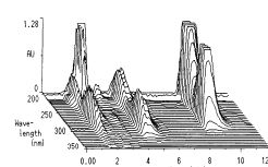
Figure 10. SFE-SFC analysis of coffee powder. A peak at about 9 min is of caffeine. Note that PDA detector was used as early as 1985 in SFC. (ref-17).
