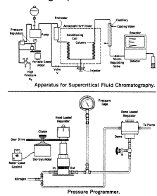
Figure 4. SFC system with pressure programming by Jentoft and Gouw in 1970. (ref-8).
