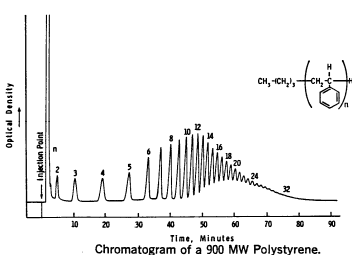
Figure 5. Separation of polystyrene 900 with pressure programming by Jentoft and Gouw in 1970. Mobile phase: n-pentane with 5% methanol. (ref-8).
